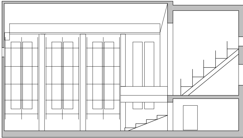
BITEF, Beograd presek R 1:200
