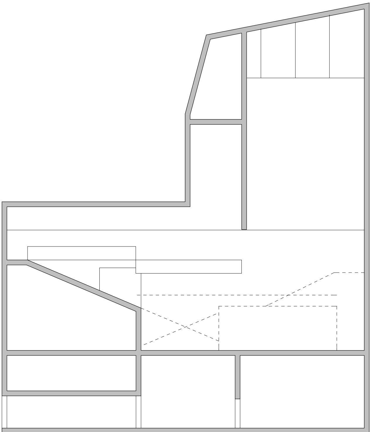
Zvezdara teatar, Beograd presek velike sale R 1:200
